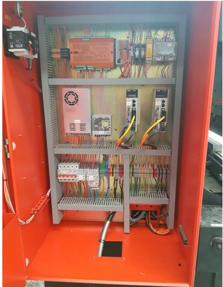
AMADA UPSTROKE
