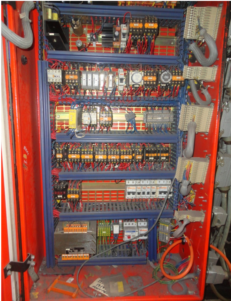
BEFORE UPGRADE AND AFTER UPGRADE iCON-1 replaces many relays and contactors
